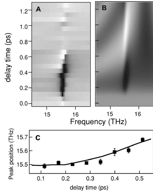
FIG. 3. Comparison of the experimental \Delta E/E data around 15.5 THz (a) with the modeled data at the same frequency range (b). Scale as in Fig. 2, but inverted for clarity, (see text for details). Panel (c) depicts the central frequency of both the experimental (squares) and modeled (solid line) data obtained from Lorentzian fits to horizontal cuts through panels (a) and (b).
